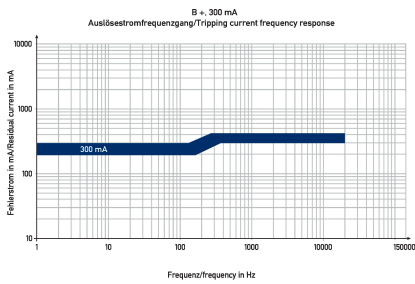
Characteristic B+ 300 mA
