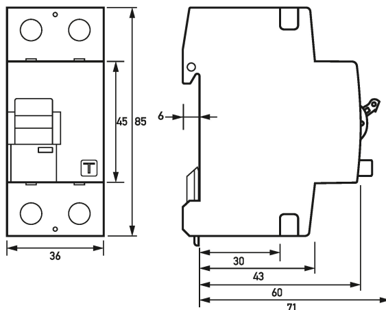
Dimensional drawing DFS 2 F, 2-pole (Group view)
