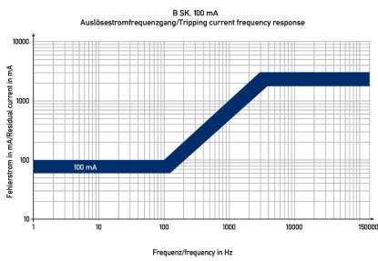
Characteristic B SK 100 mA
