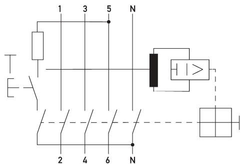
Wiring example residual current circuit-breaker DFS 4 025-4/0,10-AC R
