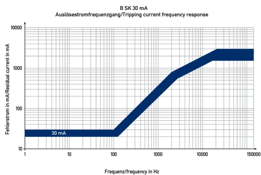
Diagrams residual current circuit-breaker DFS 2 025-2/0,03-B SK
