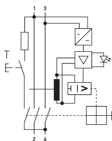
Wiring example residual current circuit-breaker DFS 2 025-2/0,03-HP
