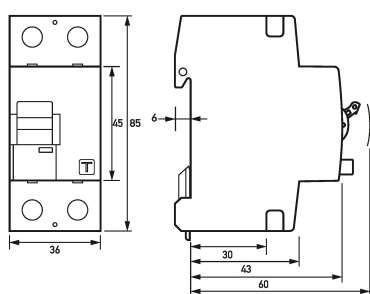
Dimensioned drawing residual current circuit-breaker DFS 2 025-2/0,03-HP
