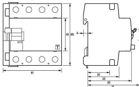
Dimensioned drawing residual current circuit-breaker DFS 4 025-4/0,01-A FT
