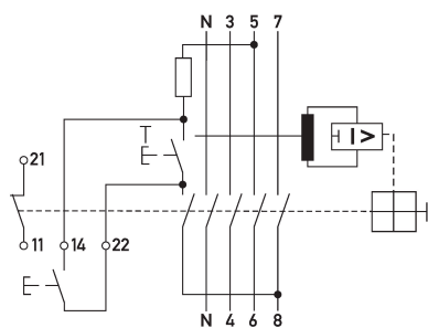
Wiring example residual current circuit-breaker DFS 4 025-4/0,01-A FT
