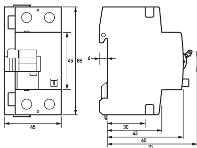
Dimensioned drawing residual current circuit-breaker DFS 2 A FT, 2-pole
