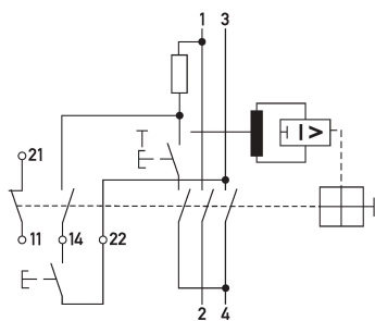
Wiring example residual current circuit-breaker DFS 2 A FT, 2-pole
