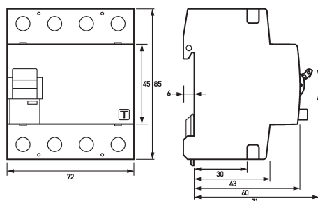
Dimensioned drawing residual current circuit-breaker DFS 4 AC, 4-pole
