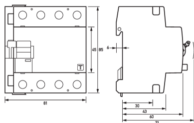
Dimensional drawing Group view
