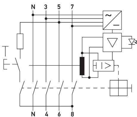
Wiring diagram DFS 4 B+ MI, 4-pole
