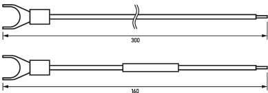
Dimensional drawing Group view
