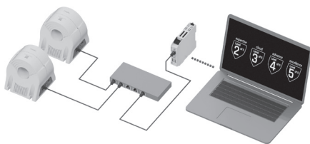
▲ Connection diagram e.Guard RCM, PoE switch, e.Guard-Gateway in Level 2
