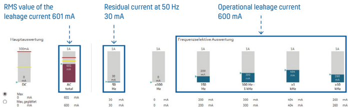
Fig. 15: Frequency-selective evaluation of the residual currents with e.Guard RCM B and allocation of the individual frequencies
