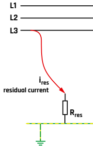
Fig. 2: AC residual current
