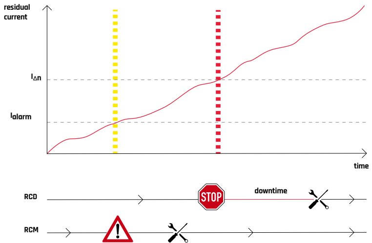
Fig. 16: Comparison between RCD and RCM
