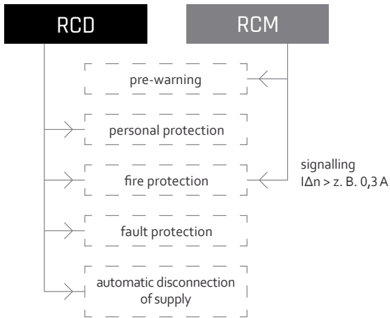
Fig. 10: compares the protection targets achieved and the degree of protection of an RCD and an RCM (without a switch-off device).
