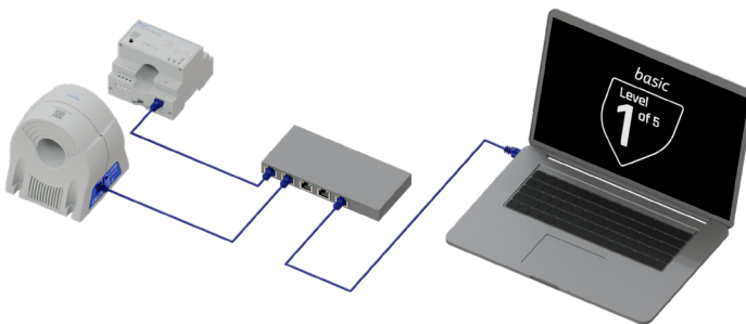
Fig. 20: e.Guard basic setup
