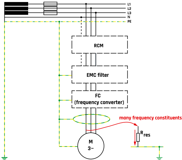
Fig. 6: Residual current with frequency mix
