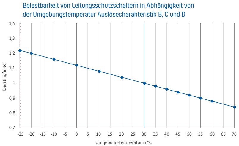
Abb. 22: Derating B, C, D Charakteristik
