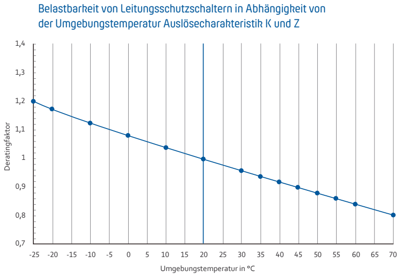
Abb. 23: Derating K, Z Charakteristik
